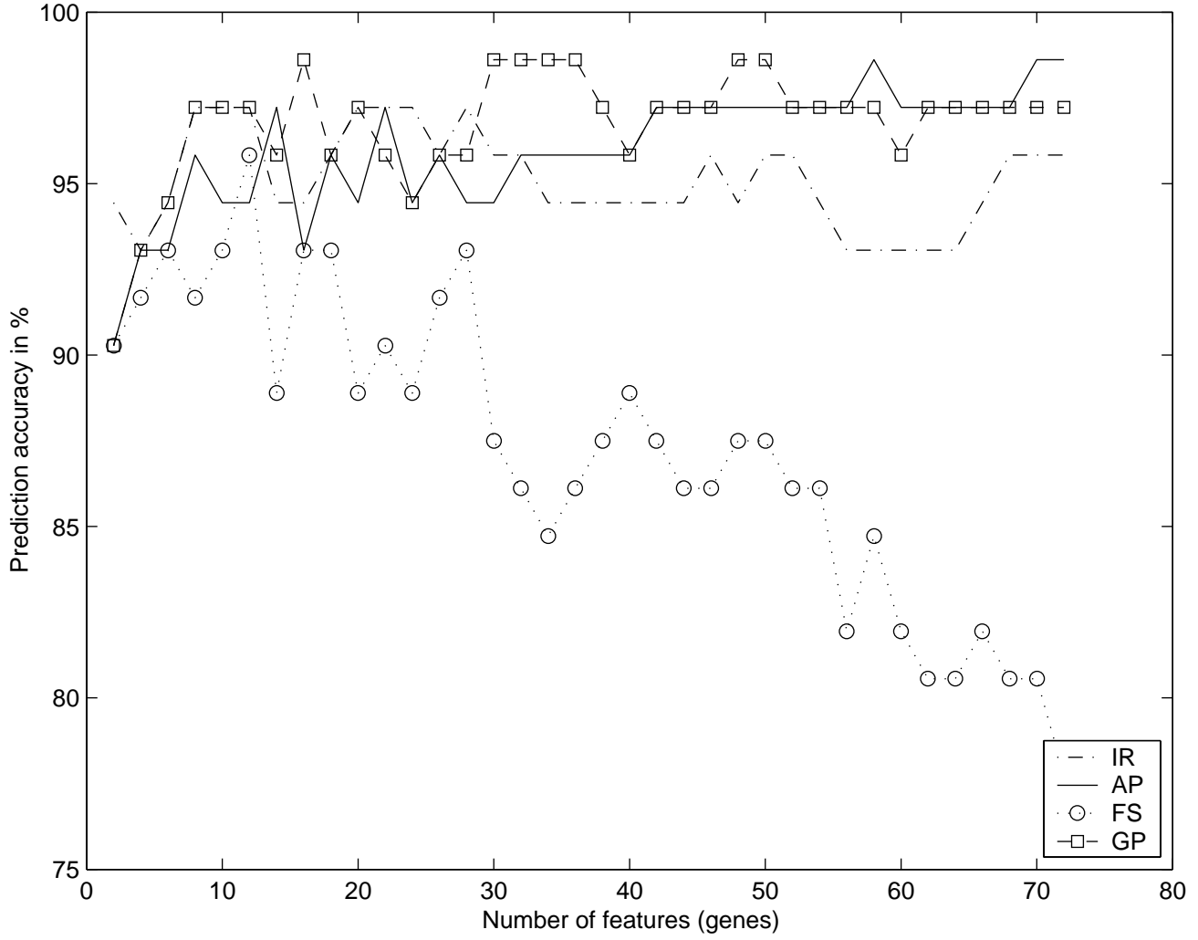
ALL/AML dataset: LOOCV and 3NN prediction
