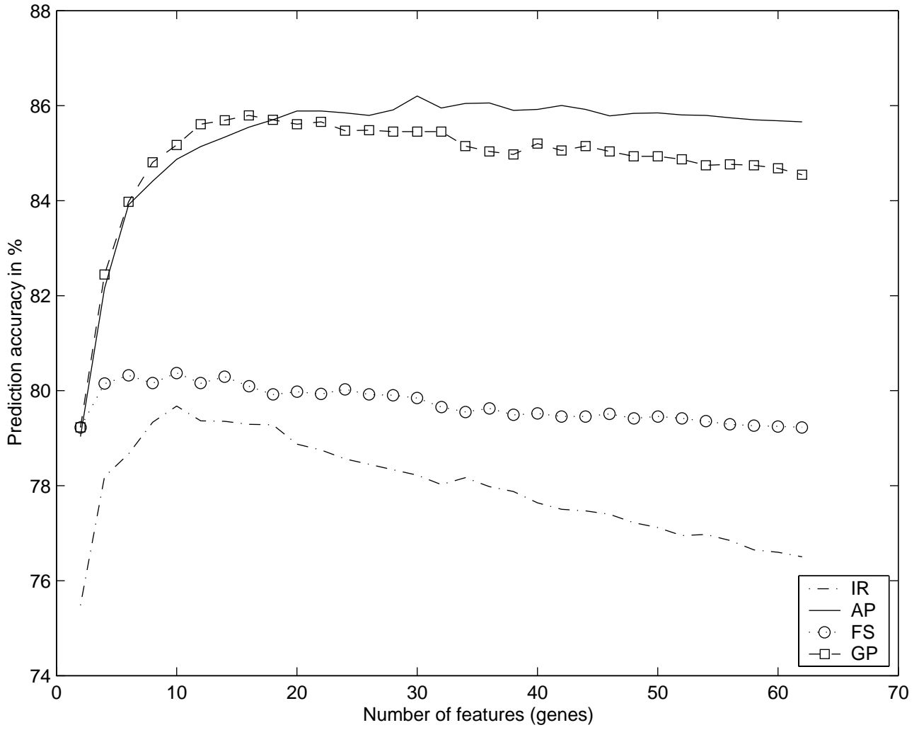
Colon dataset: L-31-OCV and FLD prediction
