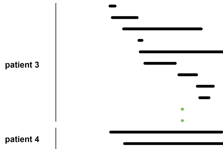
Hotspots of rearrangements in PARK2 and MACROD2 . (A) Recurrent deletions in PARK2 in patients 3 and 4. (B) Recurrent deletions and rearrangement breakpoints in MACROD2 in patient 3 and 4. Green spots indicate rearrangement breakpoints and black lines indicate deletions. Exons are depicted as vertical bars.
